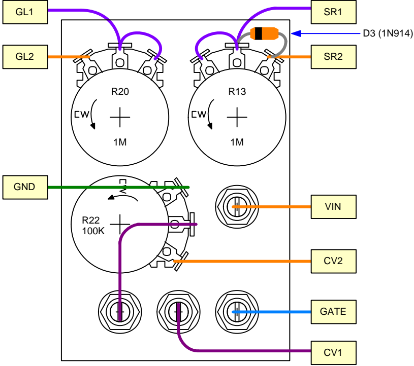
Micro Sample And Hold Rear Panel Wiring View
